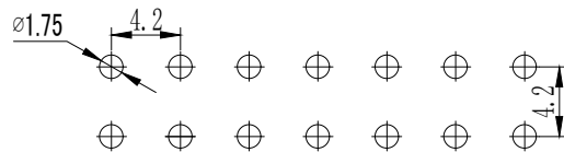
P. C. B LAYOUT
