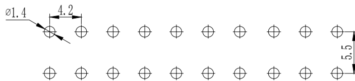
P. C. B LAYOUT
