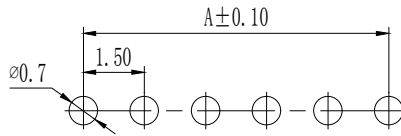
P. C. B LAYOUT
