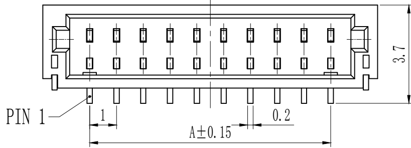
Assembly Layout
