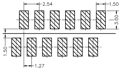
Recommended PCB Layout(Top Side)
